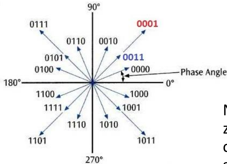
12 Phase Angles, 2 Amplitudes, 4 bits
