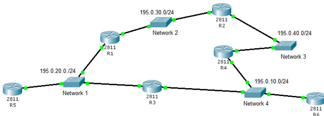
Figure 1 - Networks layout with redundant paths - RIP
