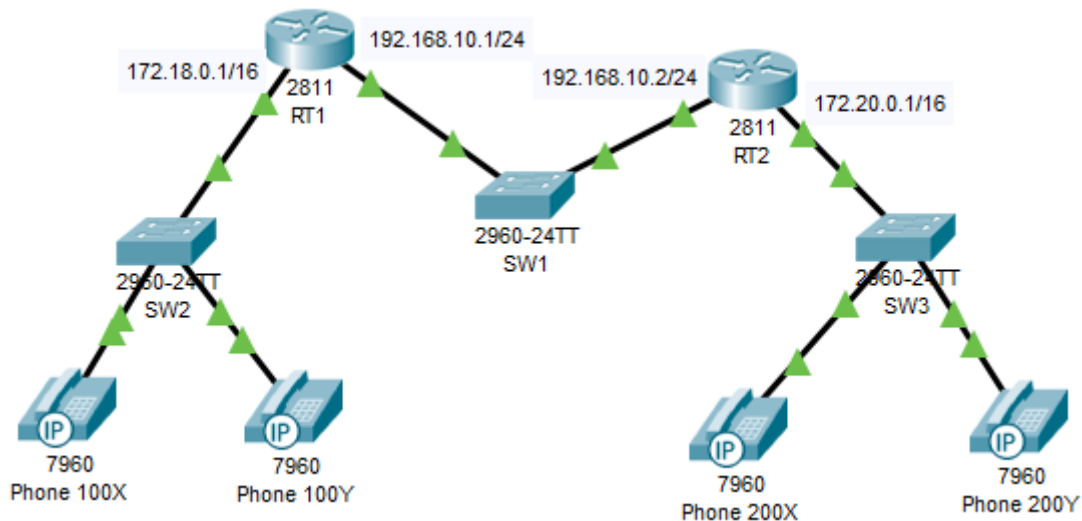
Figure 5 - VoIP layout
